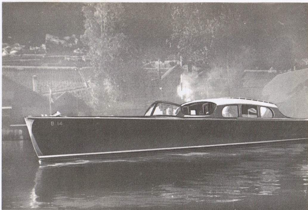
Victory II (Limousine) Länge 11 m; Motor 200 PS; Max. 45 km/h; Salon; Küche; WC.
